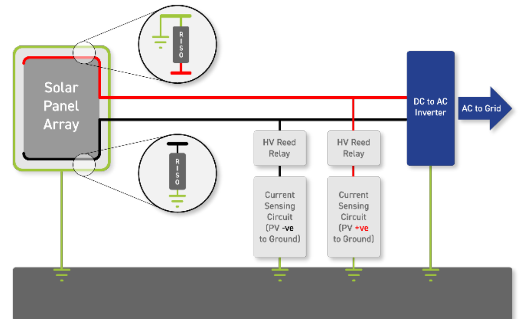
Diagram 1 The current sensing circuit includes a resistor of a known value (typically a high impedance). When the circuit is switched in, the known resistance will effectively be placed in parallel with the RISO. The current that flows through the sensing circuit can be used to calculate the RISO.
